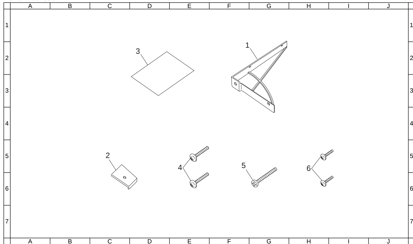
FIG. 5 ACCESSORY
