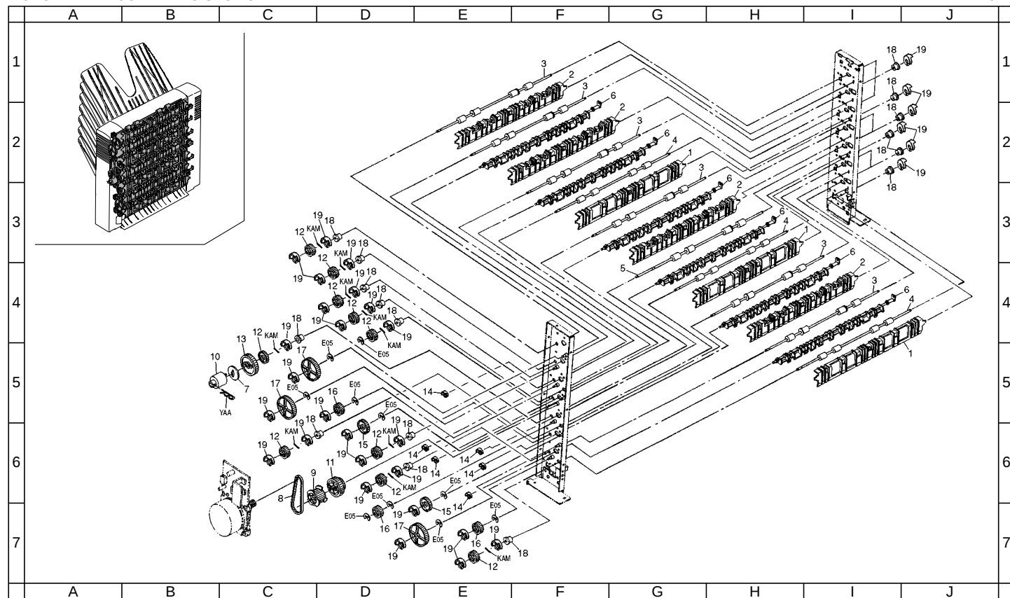
FIG. 3 PAPER CONVEYING SECTION 2
